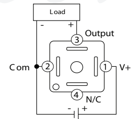
0-5VDC Output
