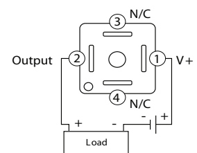
4-20mA Output
