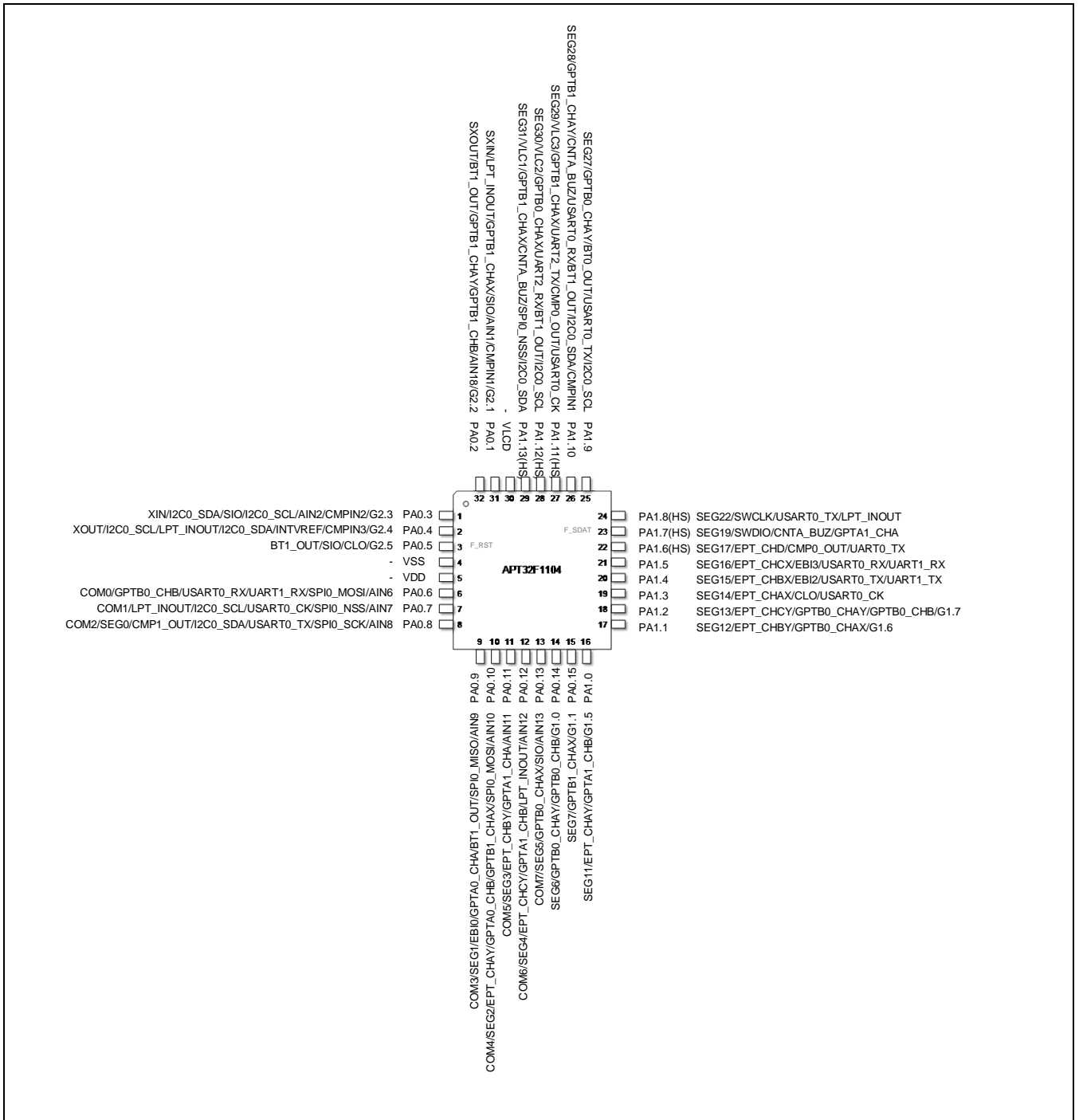
Figure 2-3 管脚定义图(32 LQFP/32 QFN)
