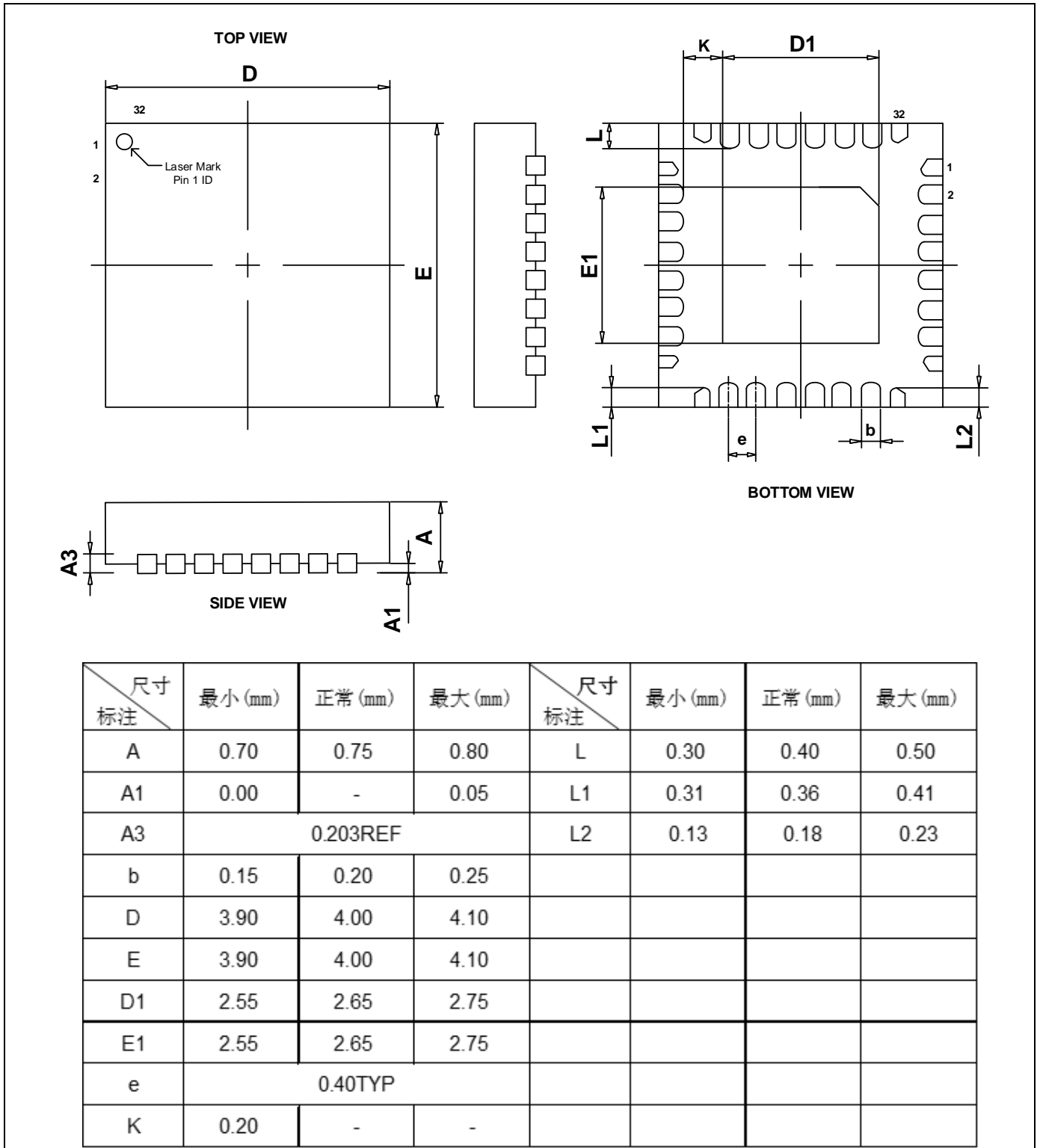
Figure 4-4 QFN32 (4x4, 0.4mm)封装尺寸
